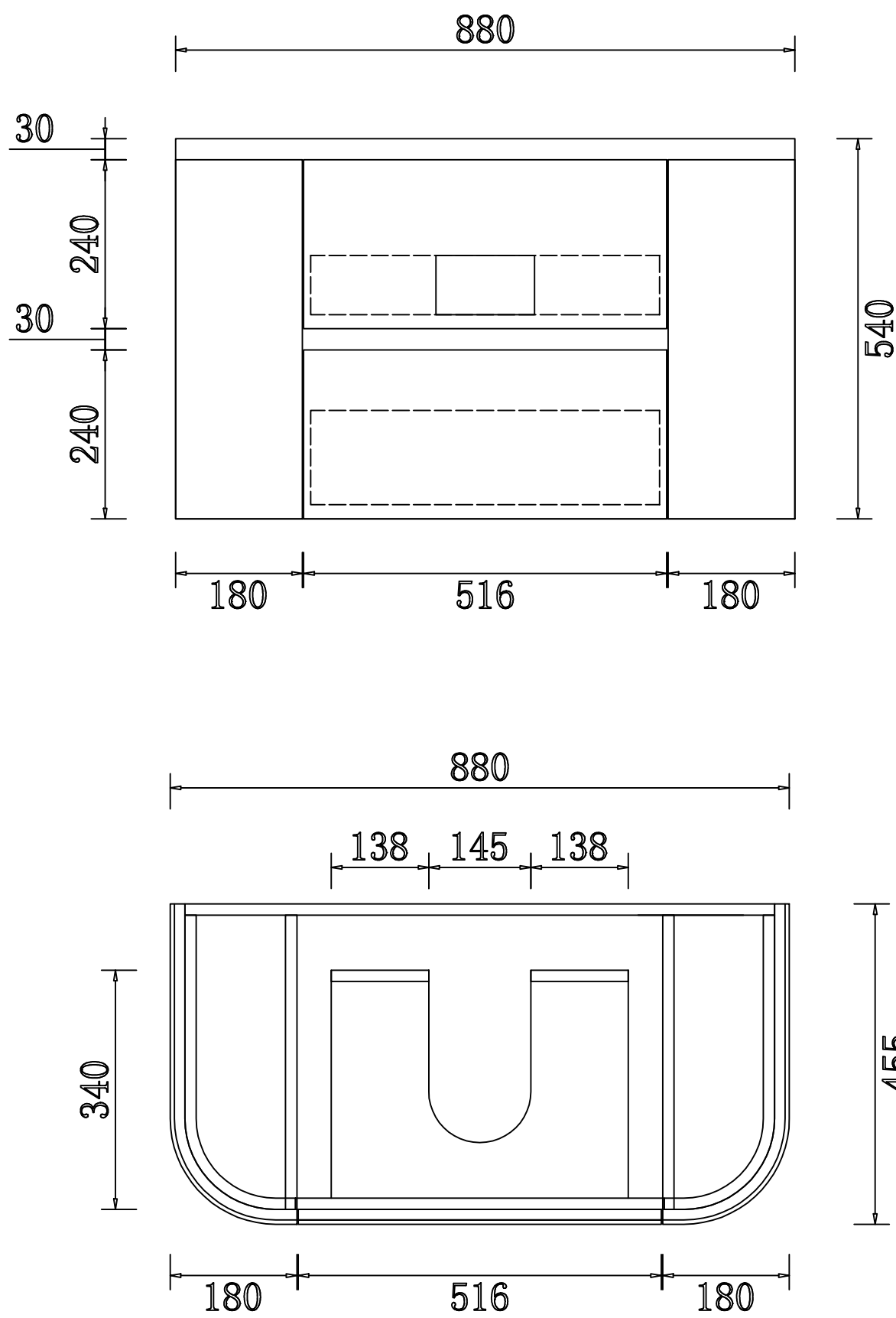
CWH68-900 SIZE: 880*455*540H
