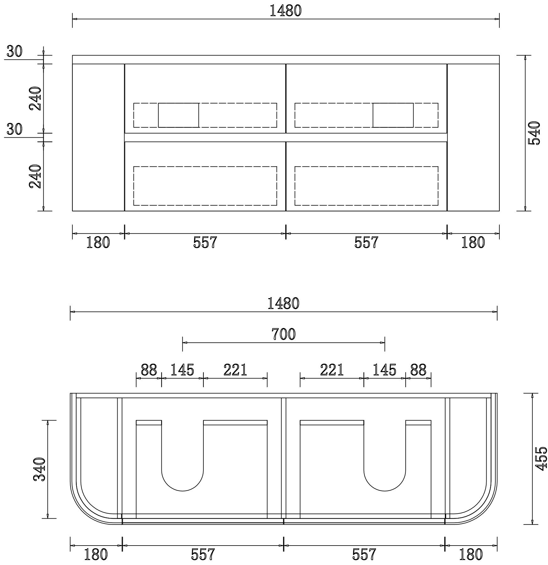
CWH68-1500D SIZE: 1480*455*540H
