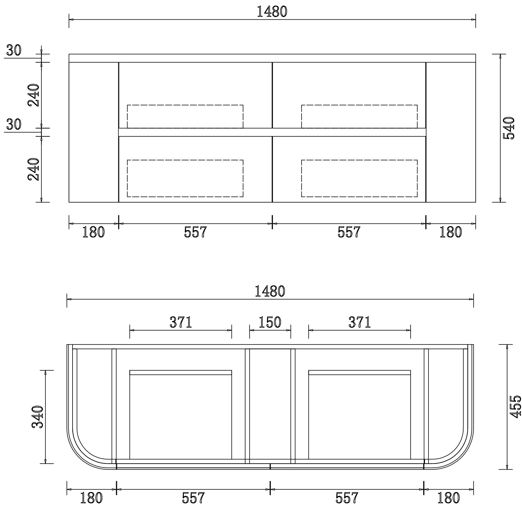
CWH68-1500S SIZE: 1480*455*540H
