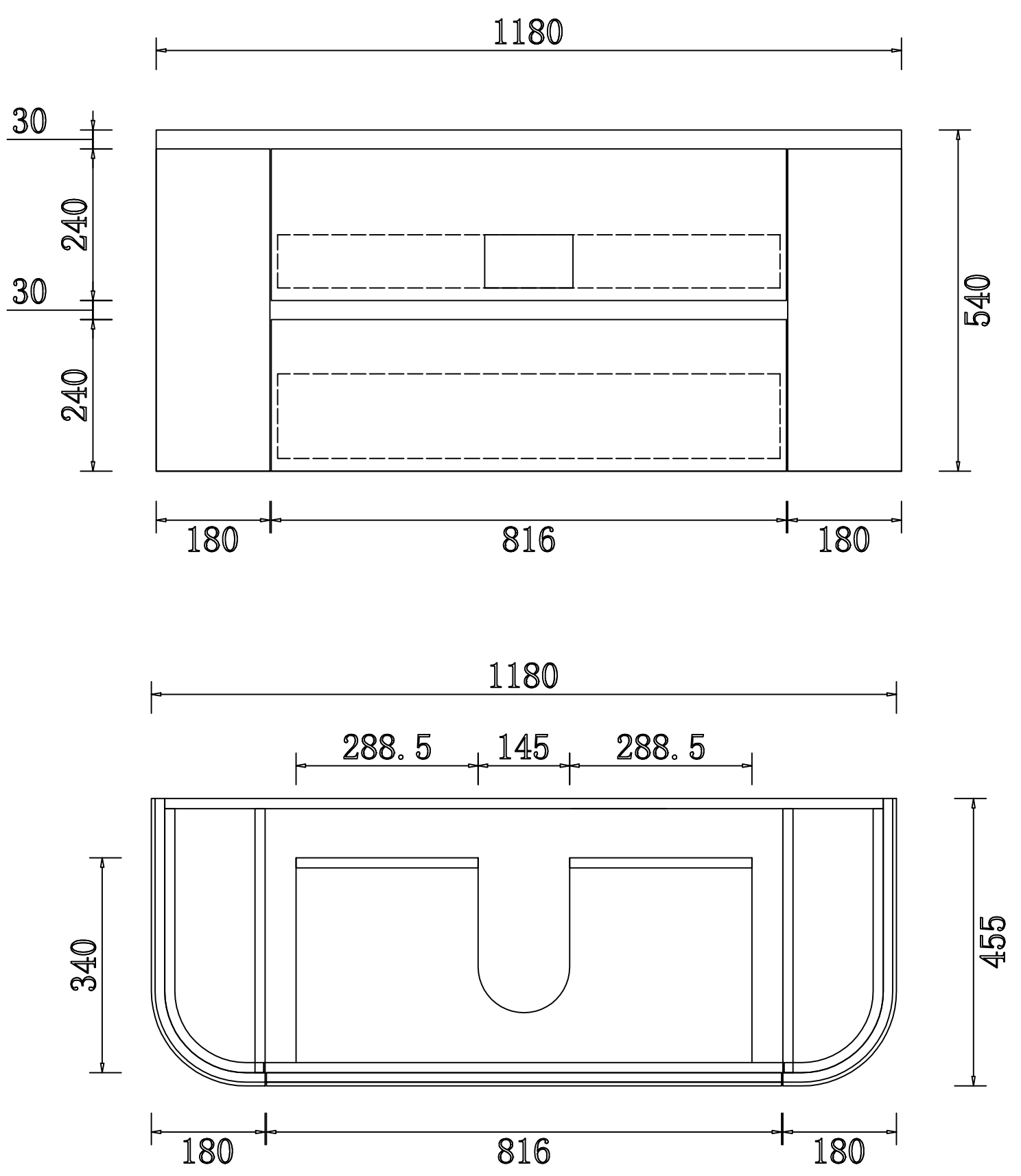
CWH68-1200 SIZE: 1180*455*540H
