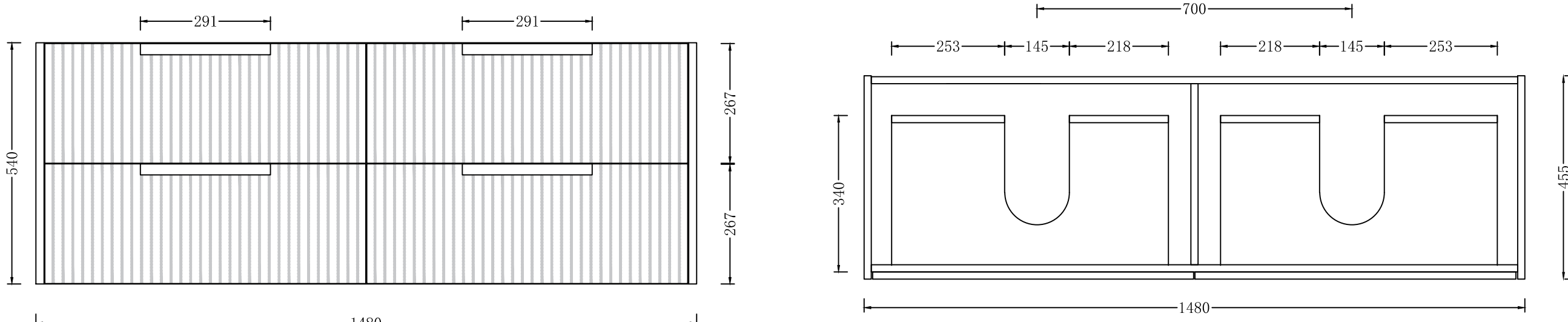
WH86-1500D-NEW SIZE: 1480*455*540H
