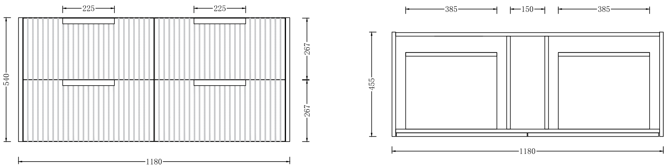
WH86-1200-NEW SIZE: 1180*455*540H
