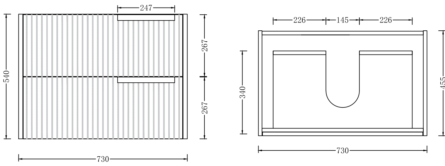
WH86-750-NEW SIZE: 730 *455*540H
