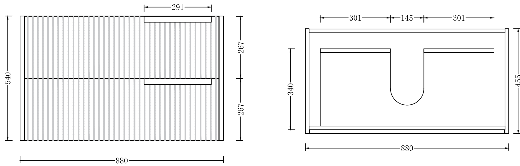
WH86-900-NEW SIZE: 880*455*540H
