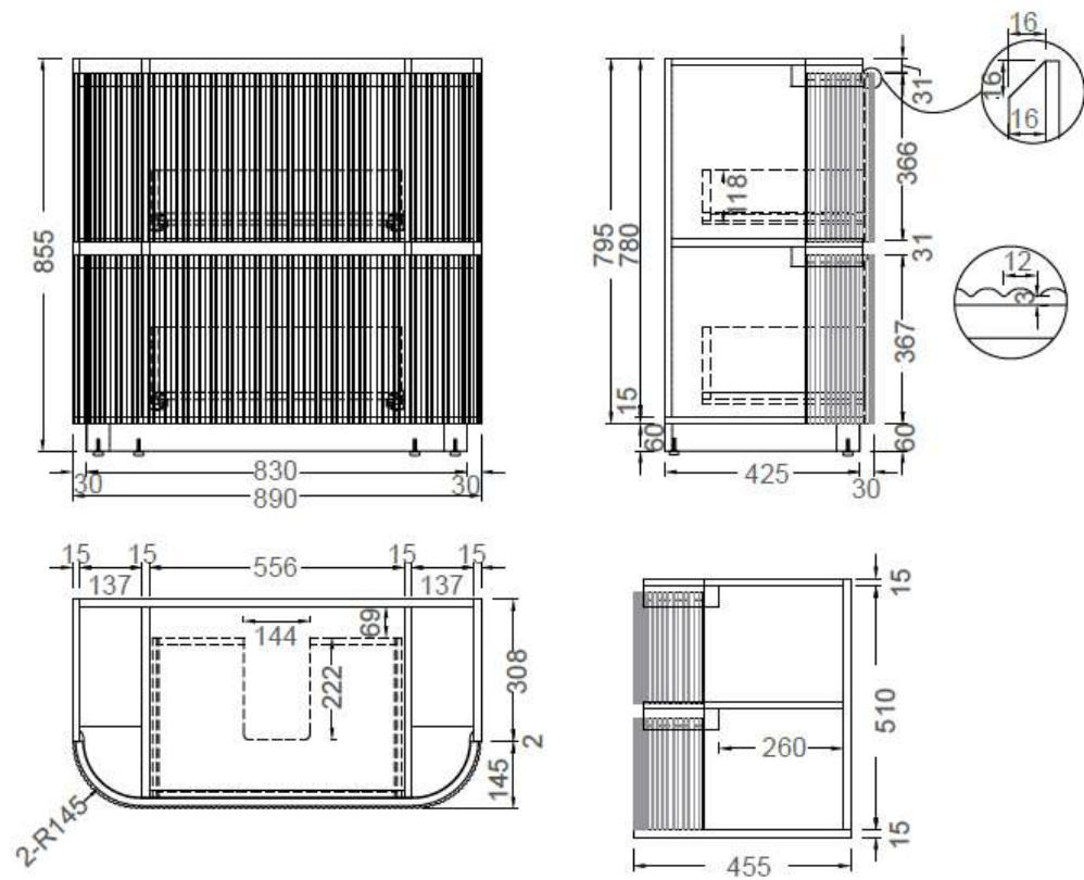
SK69-900 Size: 880x455x855Hmm
