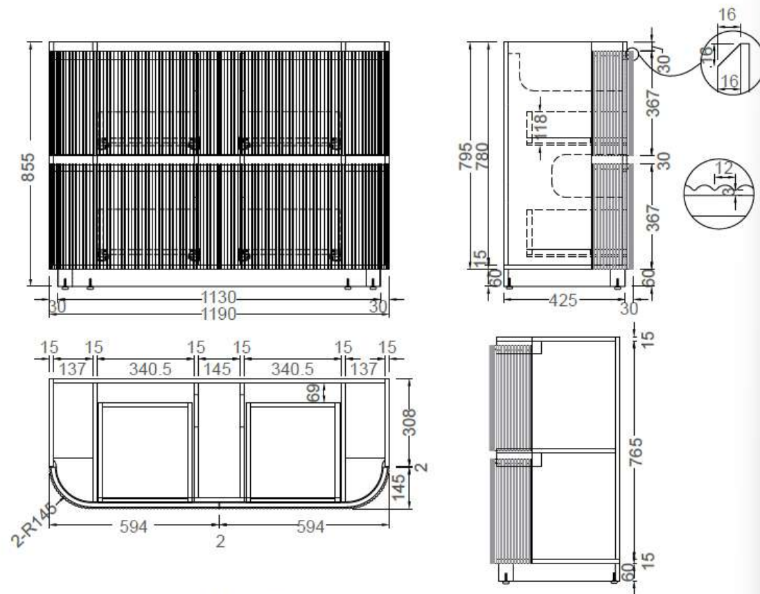
SK69-1200 Size: 1180x455x855Hmm
