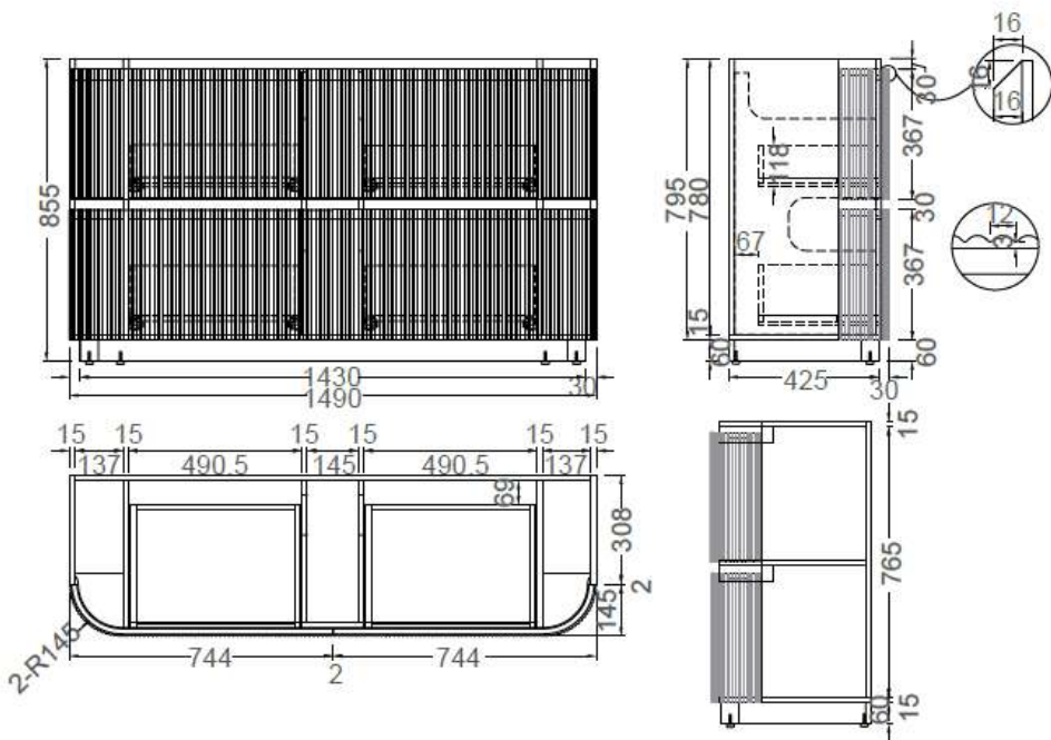
SK69-1500S Size: 1480x455x855Hmm
