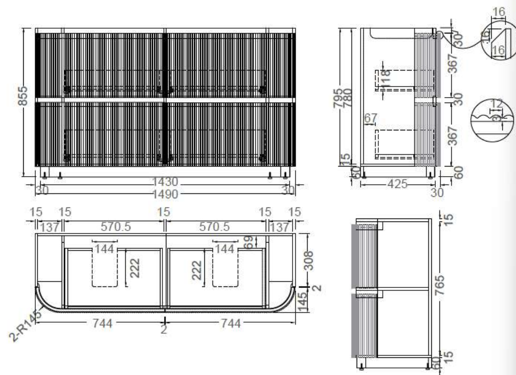
SK69-1500D Size: 1480x455x540Hmm
