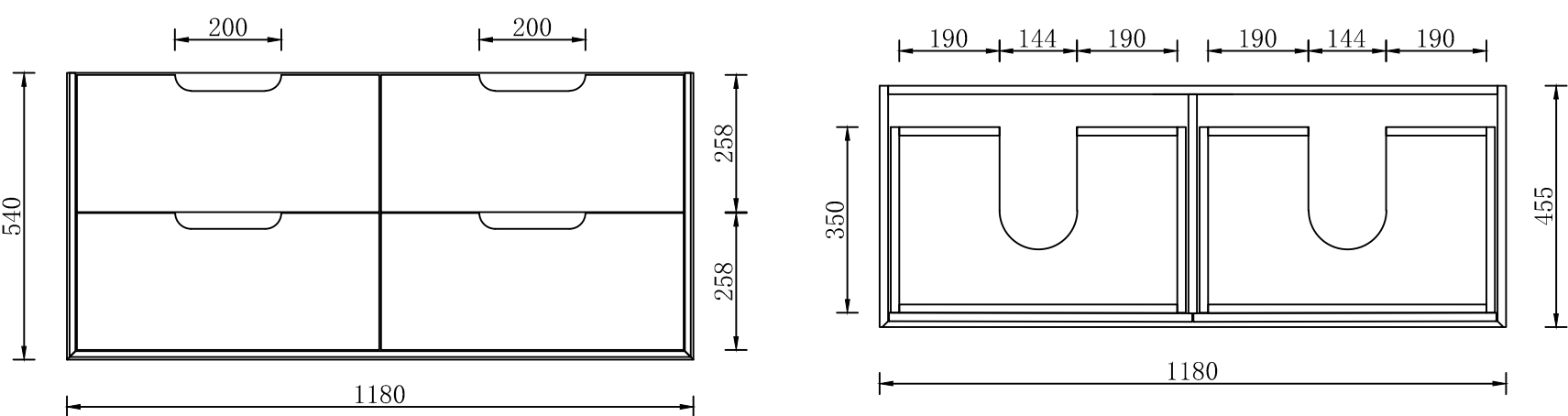
SYWH04-1200D-NEW SIZE: 1180*455*540H
