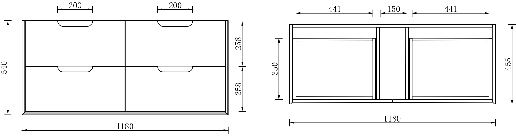
SYWH04-1200S-NEW SIZE: 1180*455*540H
