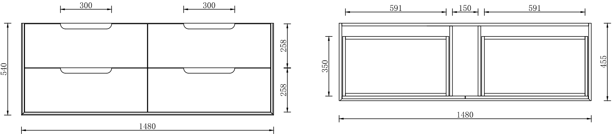
SYWH04-1500S-NEW SIZE: 1480*455*540H
