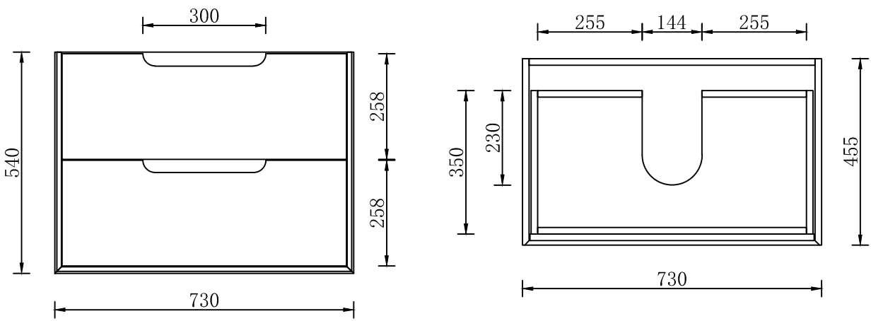
SYWH04-750-NEW SIZE: 730*455*540H
