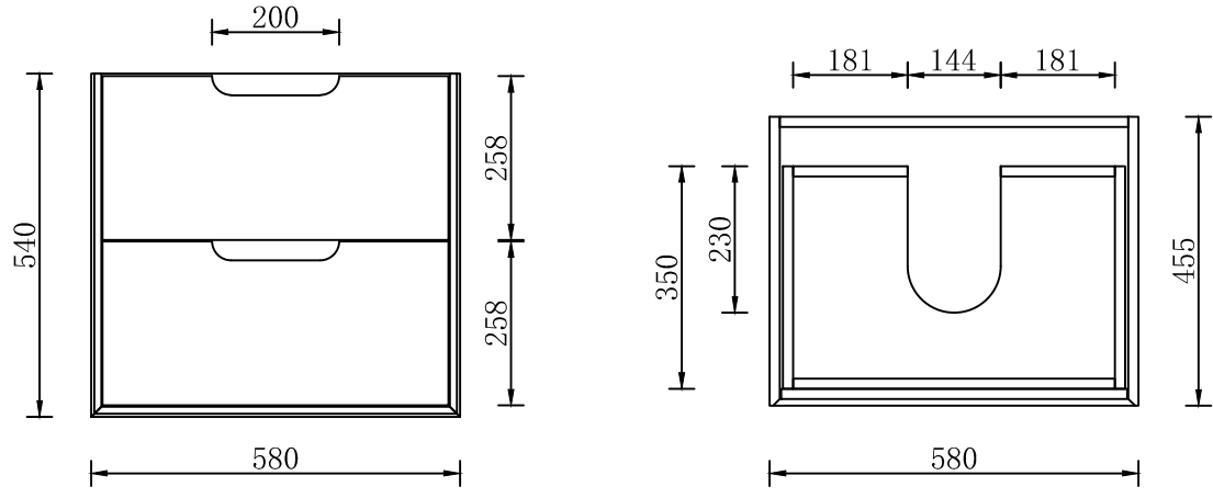
SYWH04-600-NEW SIZE: 580*455*540H
