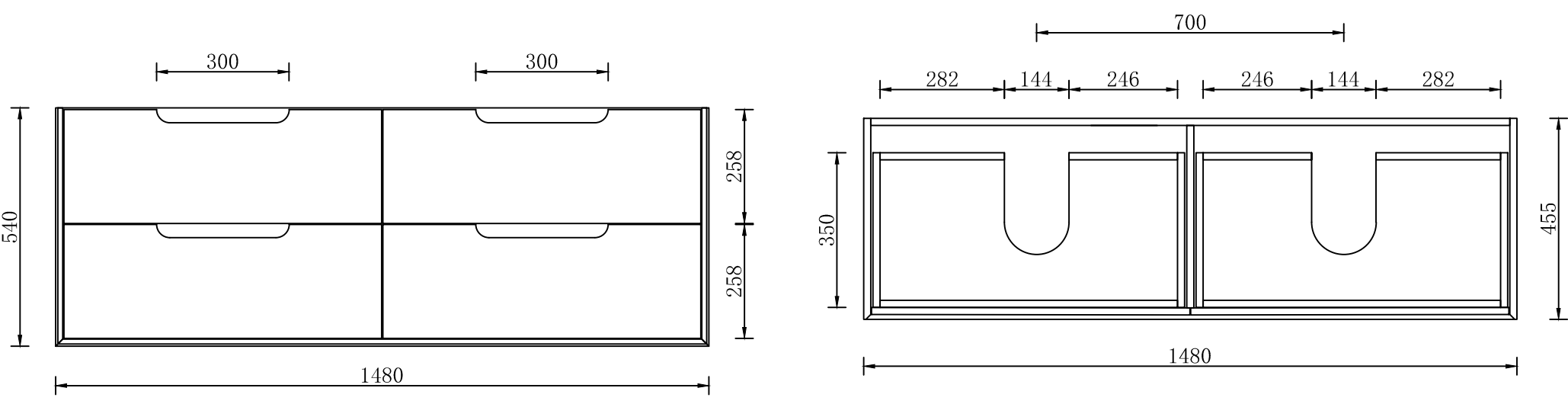
SYWH04-1500D-NEW SIZE: 1480*455*540H
