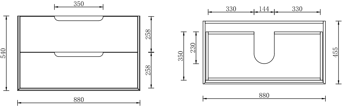
SYWH04-900-NEW SIZE: 880*455*540H
